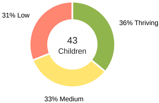
AGASSIZ - HARRISON
